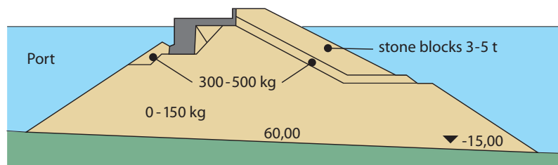
MAKARSKA BREAK WATER cross section
